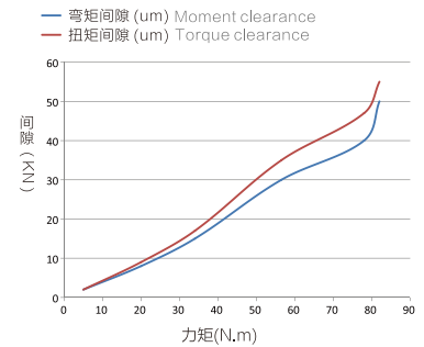
OQT-20 弯矩、扭矩变位曲线图 OQT-20 Bending moment and torque changer curve
