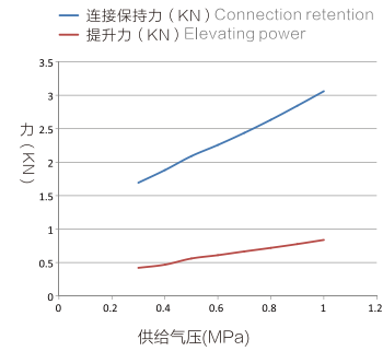
OQT-20 连接力、提升力曲线图 OQT-20 continuous relay and lifting force curve
